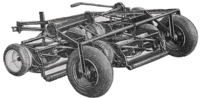
No. 21T Transport takes No. MR21-3G Mower to another job. Mower Reels do not rotate during transport - this prevents heating and distortion. Frame gives about 5" clearance and stores in upright position to save space.
