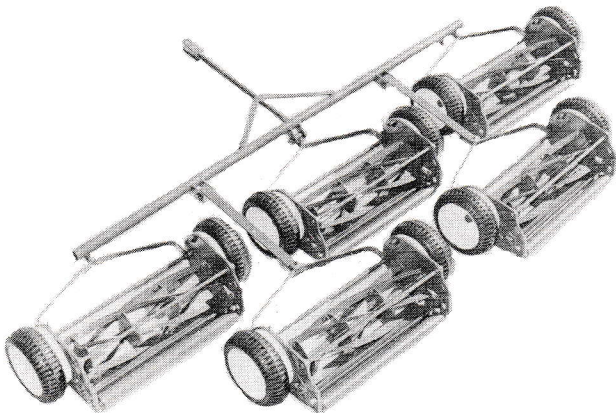
MR21-5G cutting 96" 465 lbs. The #6600 Hitch used here can also be used in the rear with UM21-3W shown above plus two MR21-1G Mowers to cut 90"
